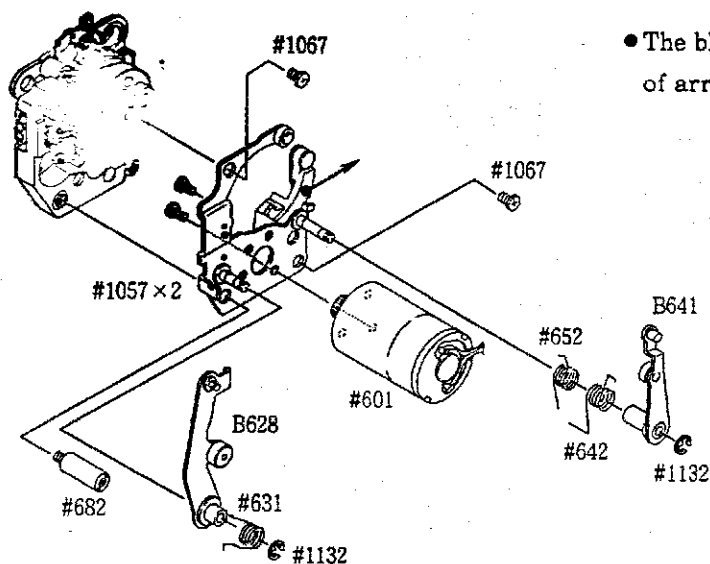
Hooking position of spring #631 Hooking position of spring #652 Hooking position of spring #642
