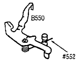
Hooking position of spring #552
