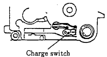
Mounting position of charge switch and arrange wires.
